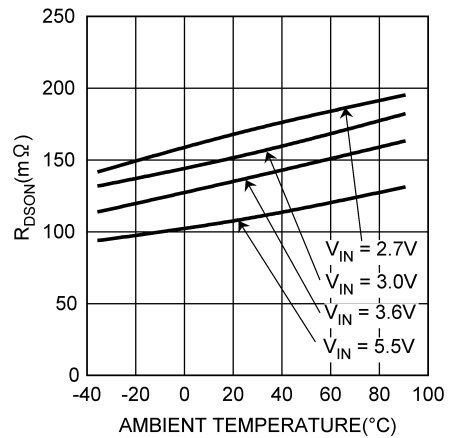
R_{DSON} vs Temperature (P-ch, I_{SW} = 200mA )
